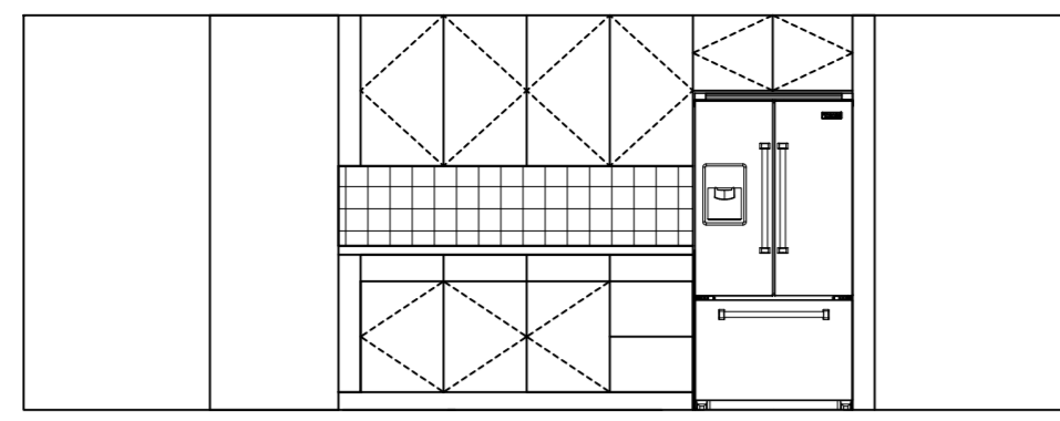
1 W. ELEVATION KITCHEN
