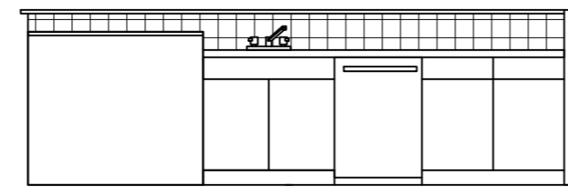
3 E. ELEVATION KITCHEN
