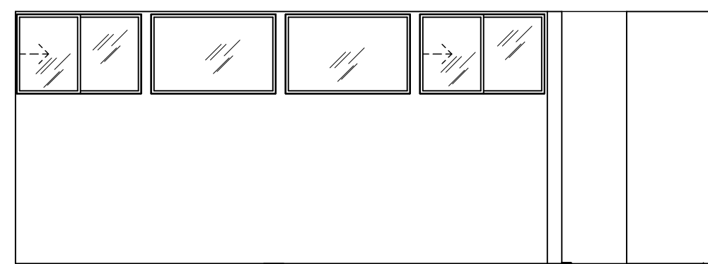
1 W. ELEVATION BEDROOM 1
